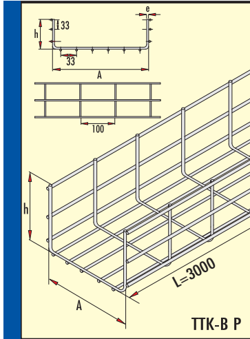
Tel Kablo Kanalı h=85 mm PASLANMAZ TEL (Cr-Ni) Wire-mesh Cable Tray h=85 mm Stainless Steel (Cr-Ni)
