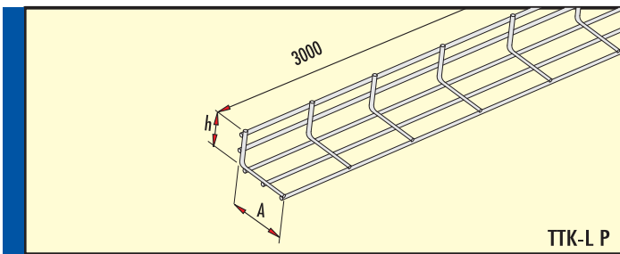
Tel Kablo Kanalı h=60 mm PASLANMAZ TEL (Cr-Ni) Wire-mesh Cable Tray h=60 mm Stainless Steel (Cr-Ni)
