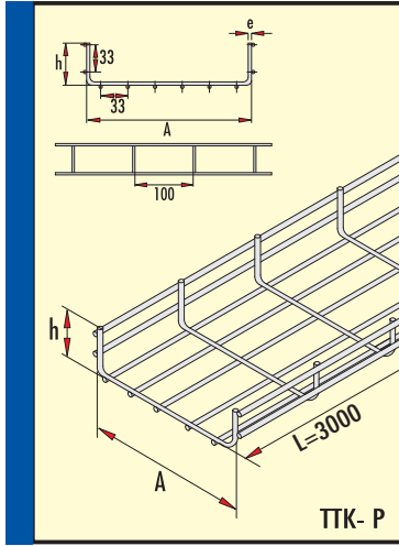
Tel Kablo Kanalı h=50 mm PASLANMAZ TEL (Cr-Ni) Wire-mesh Cable Tray h=50 mm Stainless Steel (Cr-Ni)
