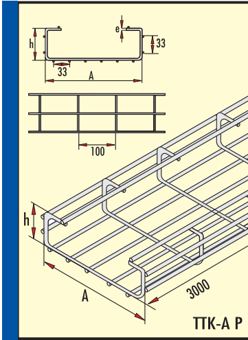
Tel Kablo Kanalı h=60 mm PASLANMAZ TEL (Cr-Ni) Wire-mesh Cable Tray h=60 mm Stainless Steel (Cr-Ni)
