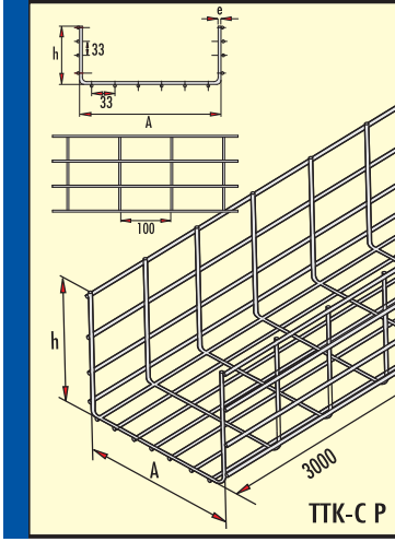
Tel Kablo Kanalı h=120 mm PASLANMAZ TEL (Cr-Ni) Wire-mesh Cable Tray h=120 mm Stainless Steel (Cr-Ni)
