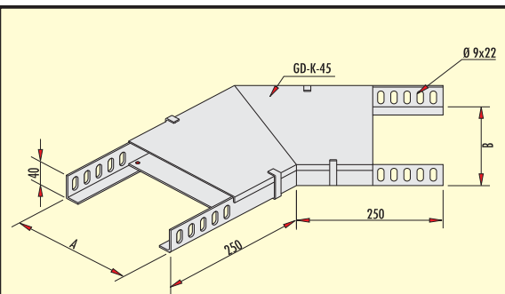
GD-K-45 P
