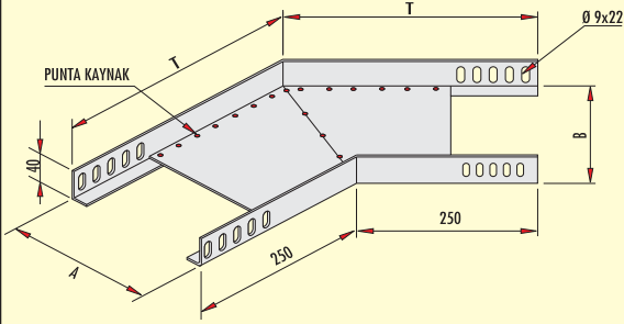
GD-45 P
