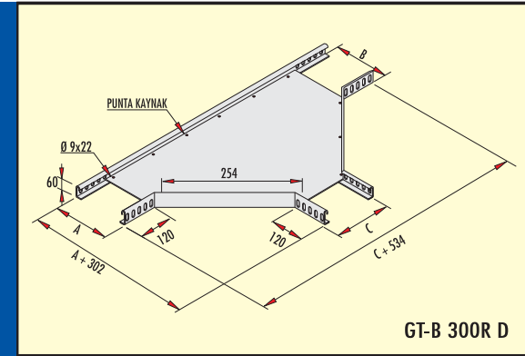
GT-B D
