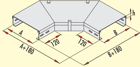
GMID-K P
