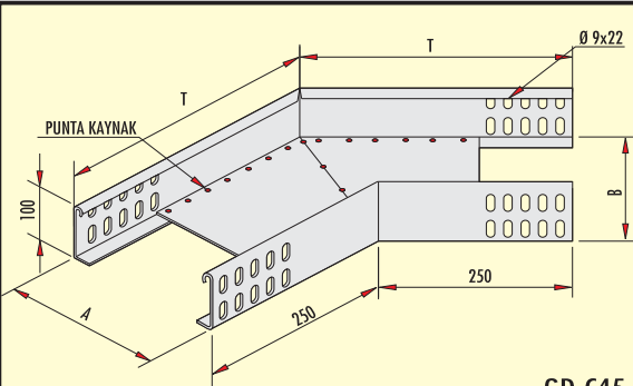
GD-C45 P
